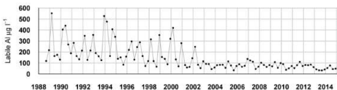
Figure 13: Labile aluminium levels in Loch Grannoch from 1988 to 2015 (taken from The
